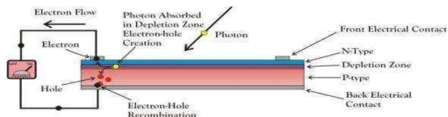
Gambar 2.5 Prinsip Kerja Panel Surya
