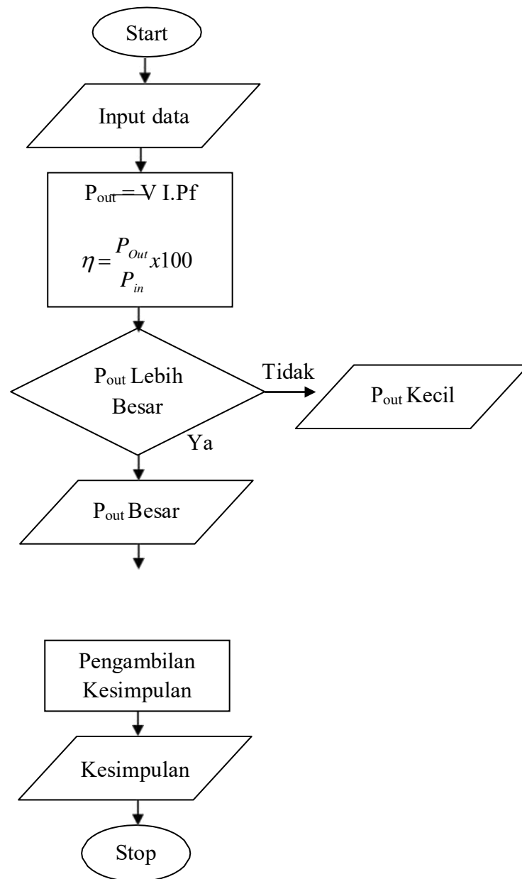
Gambar 3.1 Flowchart Penelitian
