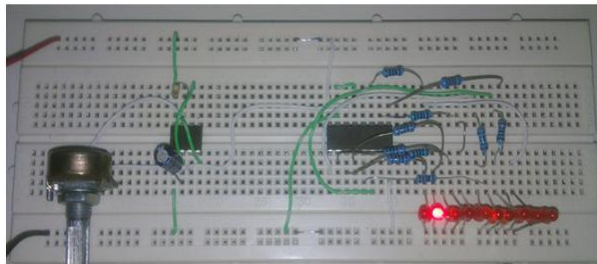
Gambar 2.8 Breadboard
