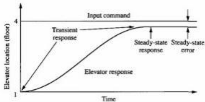
Gambar 2.2 Elevator Response Sumber : Agung Rismawan(2015)
