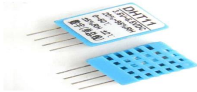
Gambar 2.6 sensor DHT11
